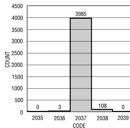
Shorted Input Histogram, 3.2V Range
